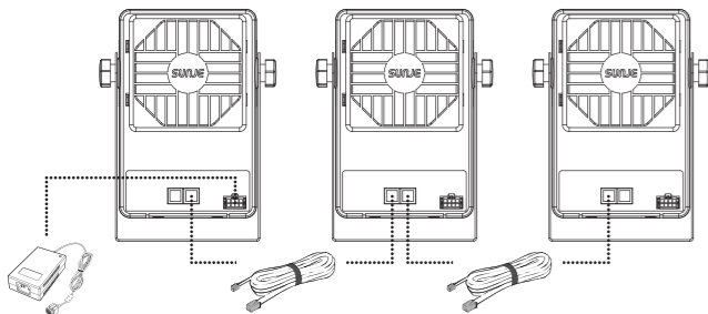
Adapter (1.5m) Extension Cable (1m)_Option Extension Cable (1m)_Option Output : DC 24V, 2.5A
