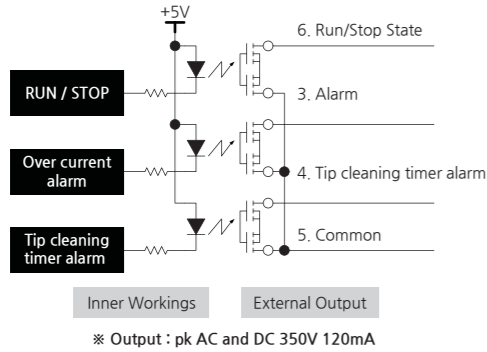
Circuit(Photo Relay Output)
